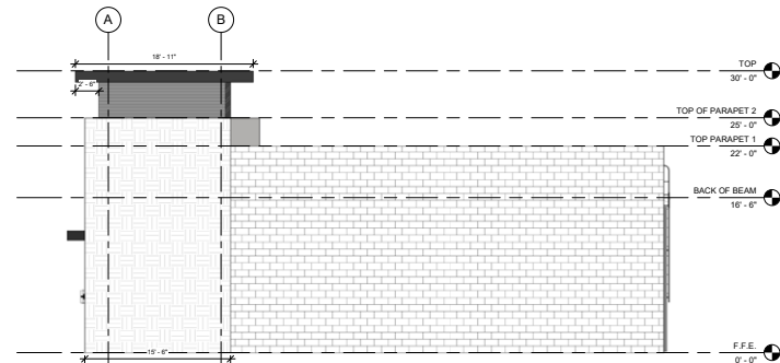
3 RIGHT ELEV. 3/16" = 1'-0"
