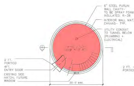
FUTURE SILO STUDY: LEVEL 1
