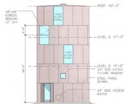
ELEVATION: FRONT
