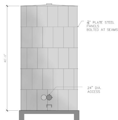
1. EXISTING ELEVATION REAR
