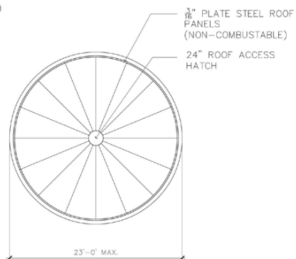
3. SILO ROOF PLAN
