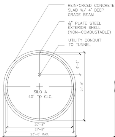
2. SILO FOOTPRINT
