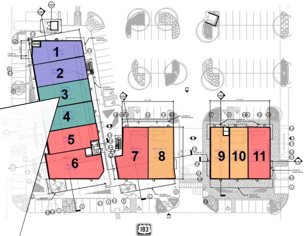
1st Floor
