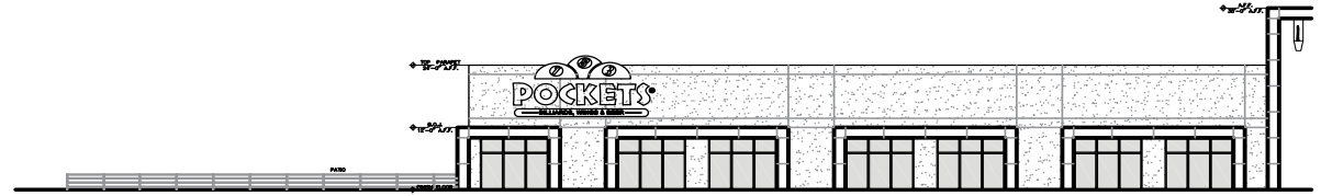
POCKETS NORTH ELEVATION SCALE: 1/8" = 1' - 0"
