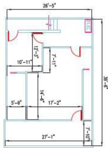
BASEMENT ±1,049 Usable Square Footage
