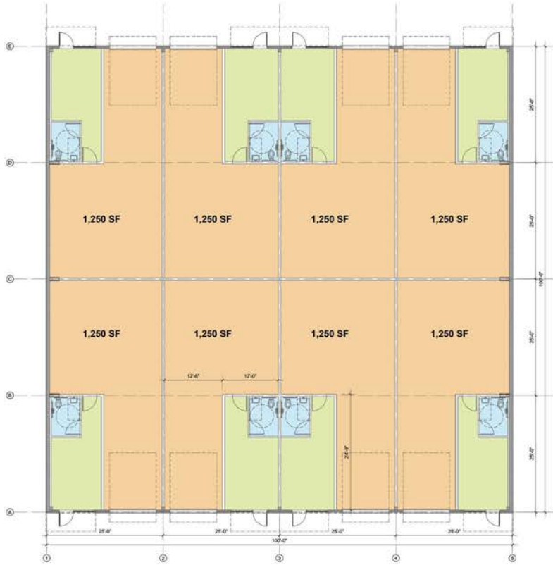
BUILDING PLAN "A" & "C"
