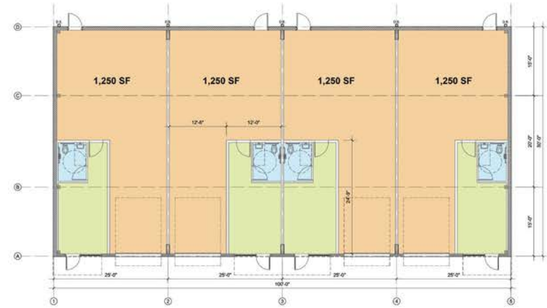
BUILDING PLAN "B" & "D"
