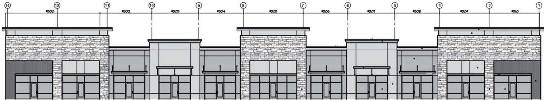
North Elevation
