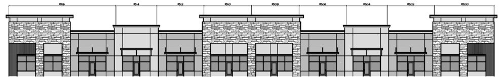
North Elevation
